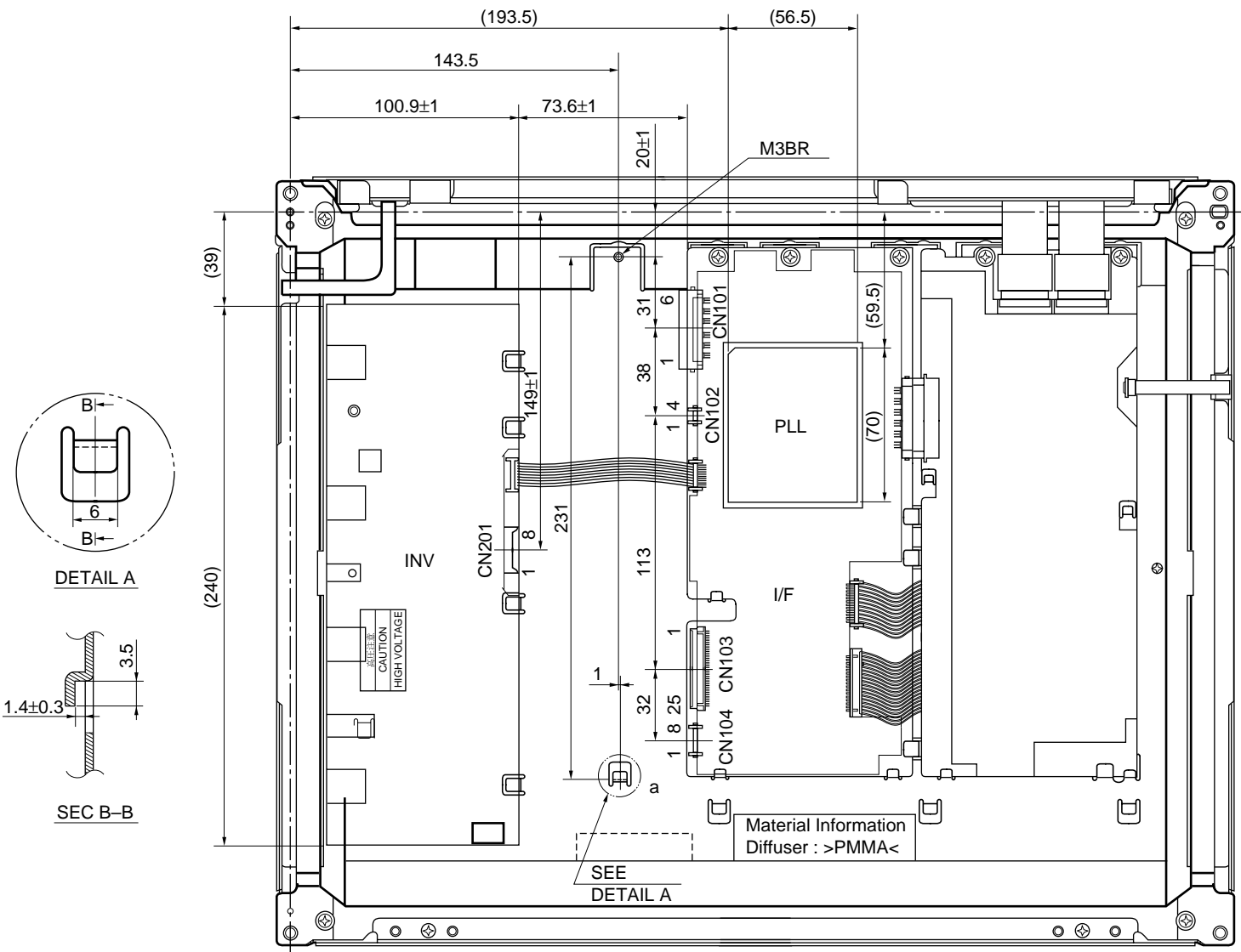
OUTLINE DRAWING: Rear View (Unit: mm)
